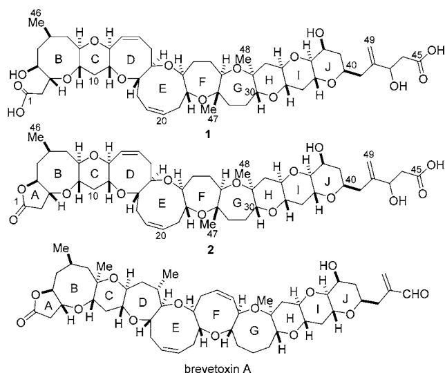
Figure 1. Structures of brevisulcatic acids-1 ( 1 ) and -4 ( 2 ) and brevetoxin A.
